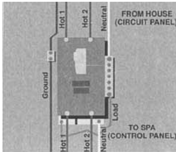
Figure 2. GFCI Hook-Up.
