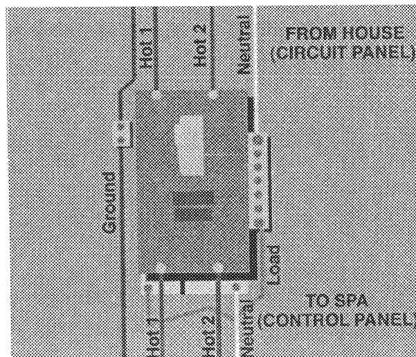
Figure 2. GFCI Hook-Up
