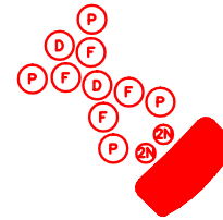
AAT (OPT19-AAT10) SEAT JET LAYOUT
